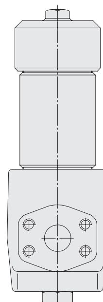
Filter with filterbowl in two-part style for element change from the top
