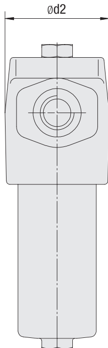
Threaded connection
