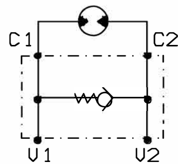
Hydraulic Symbol
