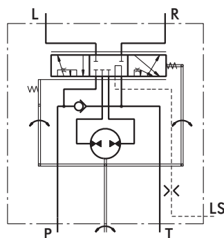
Closed Center - Non Reaction Static Signal - HKU.../5T
